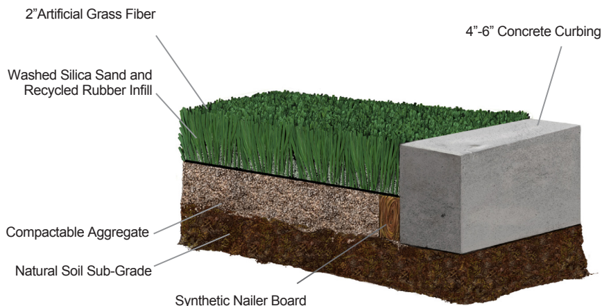
Edge Detail: Lumber or Nail Board 2"-4" Treated lumber or synthetic wood nailer board (not supplied by EasyTurf)
